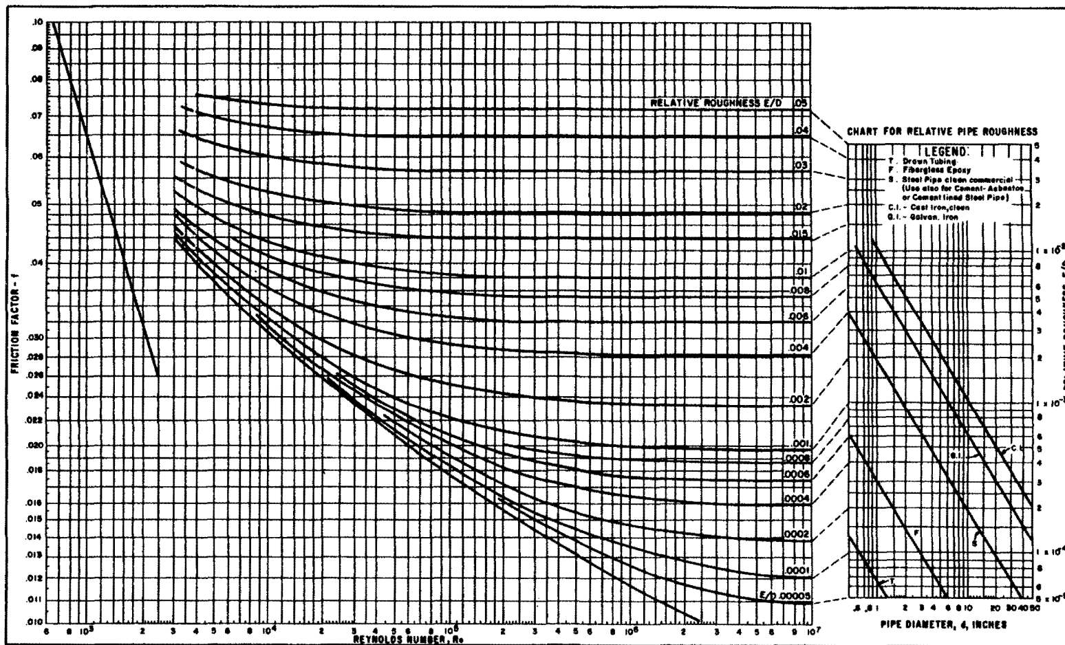
FIGURE 2.3 FRICTION FACTOR CHART (Modified Moody Diagram)
